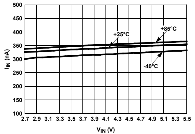
FIGURE 44. I_{IN} vs V_{IN} OVER-TEMPERATURE
