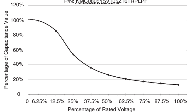
CAPACITANCE CHANGE AS FUNCTION OF APPLIED VOLTAGE (VDC)
