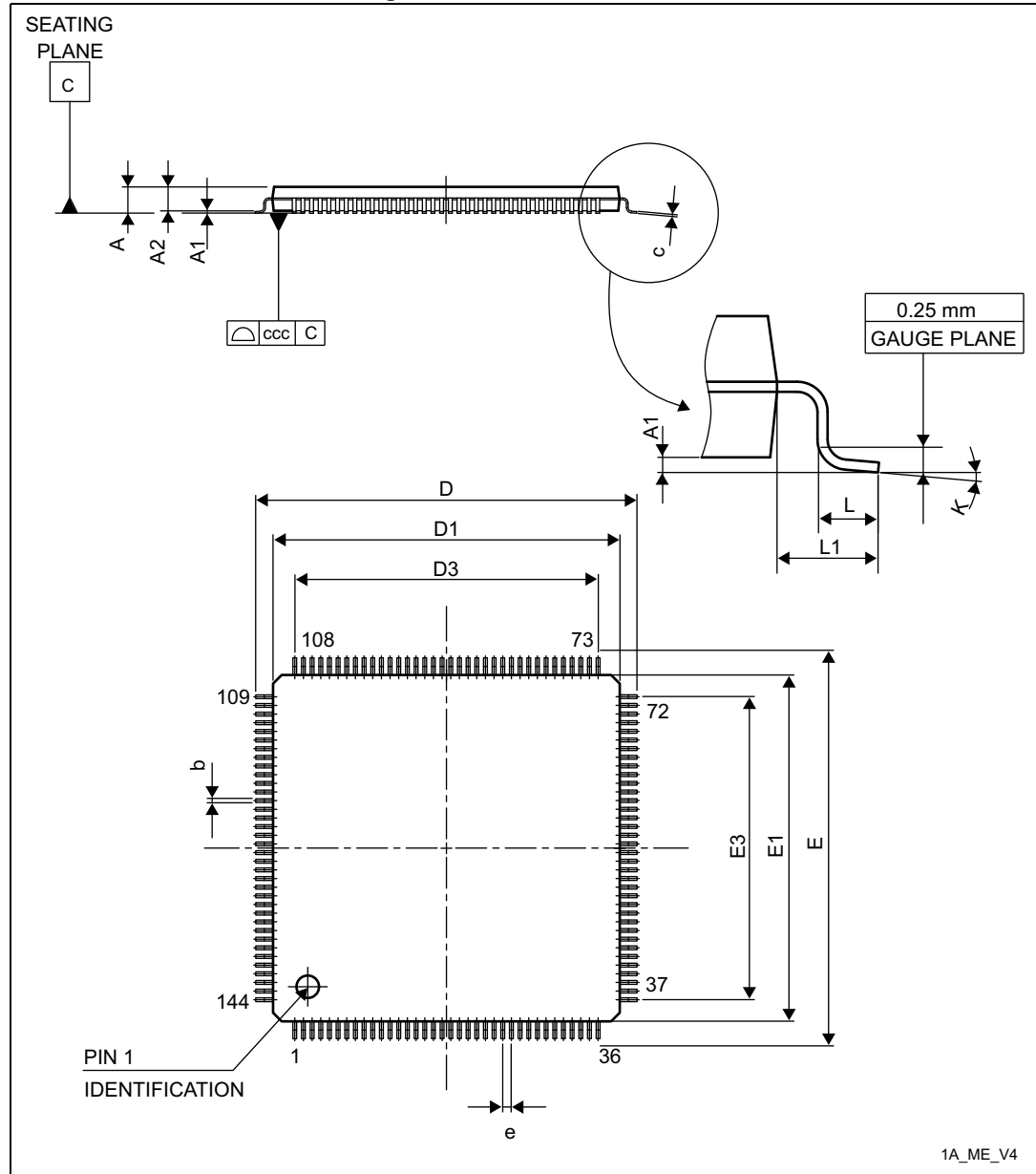
Figure 89. LQFP144 outline
