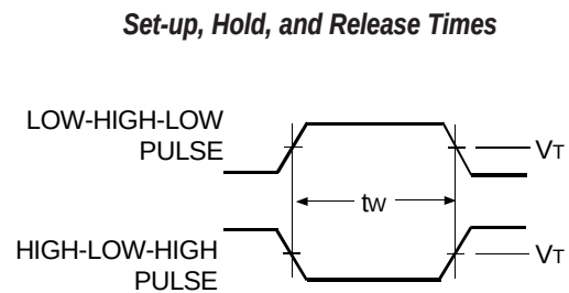
Pulse Width
