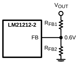
Figure 22. Setting V_{OUT}
