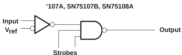
Figure 13. Single-Ended Operation
