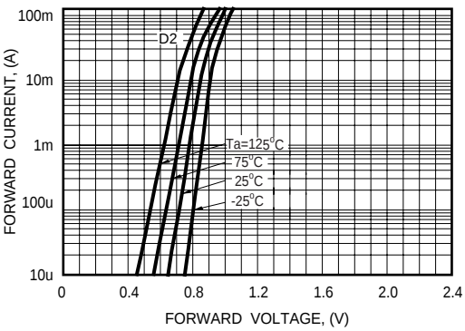
FIG. 2 - FORWARD CHARACTERISTICS
