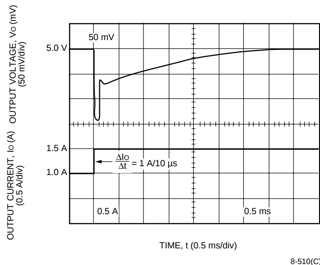
Figure 10. MW010A Typical Output Voltage Waveform for a Step Load Change from 50% to 75% of I_{o, \text{max}} ; V_I = 48\text{ V} ; T_A = 25\text{ }^\circ\text{C}
