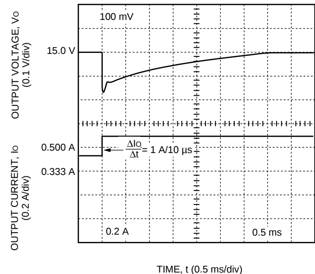
Figure 12. MW010C Typical Output Voltage Waveform for a Step Load Change from 50% to 75% of I_{o, \text{max}} ; V_I = 48\text{ V} ; T_A = 25\text{ }^\circ\text{C}
