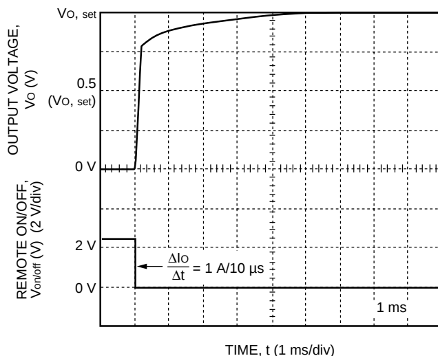
Figure 16. MW010A Typical Output Voltage Start-Up Waveform with Remote On/Off; I_o = 0.8 (I_{o,max}) ; V_i = 48 \text{ V} ; T_A = 25^\circ \text{C}
