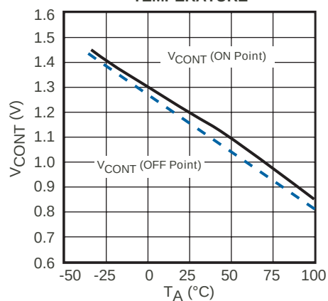
ON / OFF KNEE VOLTAGE vs. TEMPERATURE
