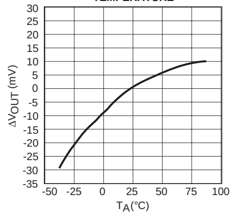
TK11150 OUTPUT VOLTAGE vs. TEMPERATURE
