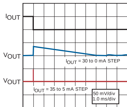
LOAD TRANSIENT 4
