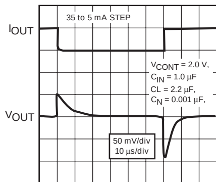
LOAD TRANSIENT 1
