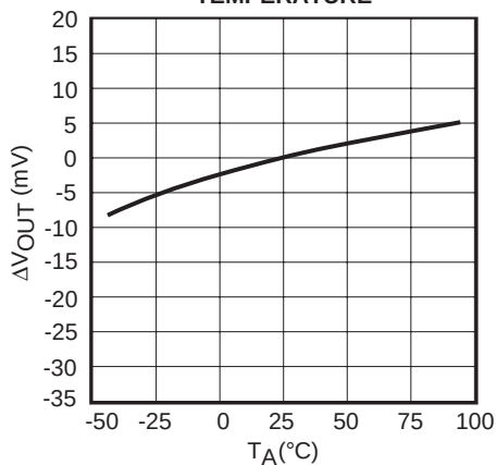
TK11120 OUTPUT VOLTAGE vs. TEMPERATURE
