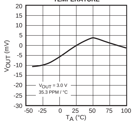
TK11130 OUTPUT VOLTAGE vs. TEMPERATURE
