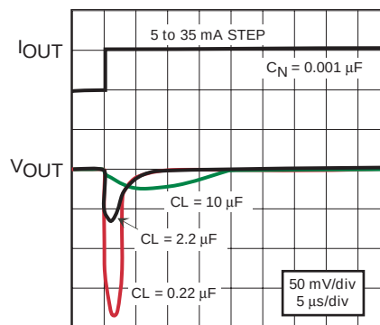
LOAD TRANSIENT 3
