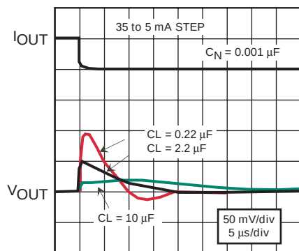
LOAD TRANSIENT 2
