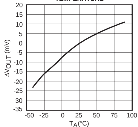
TK11140 OUTPUT VOLTAGE vs. TEMPERATURE
