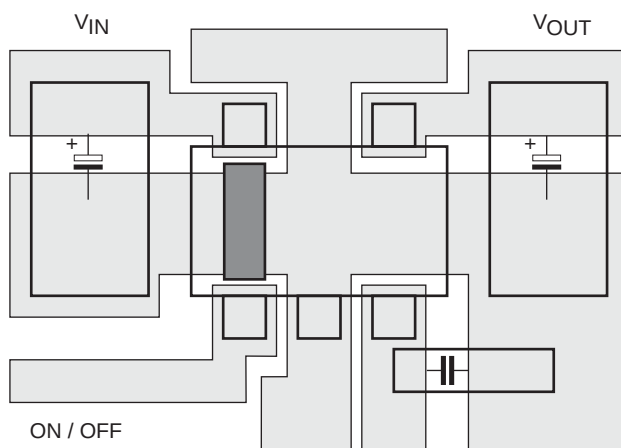
SOT23-5 BOARDLAYOUT
