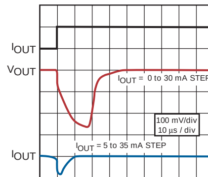
LOAD TRANSIENT 5
