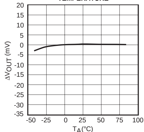
TK11115 OUTPUT VOLTAGE vs. TEMPERATURE
