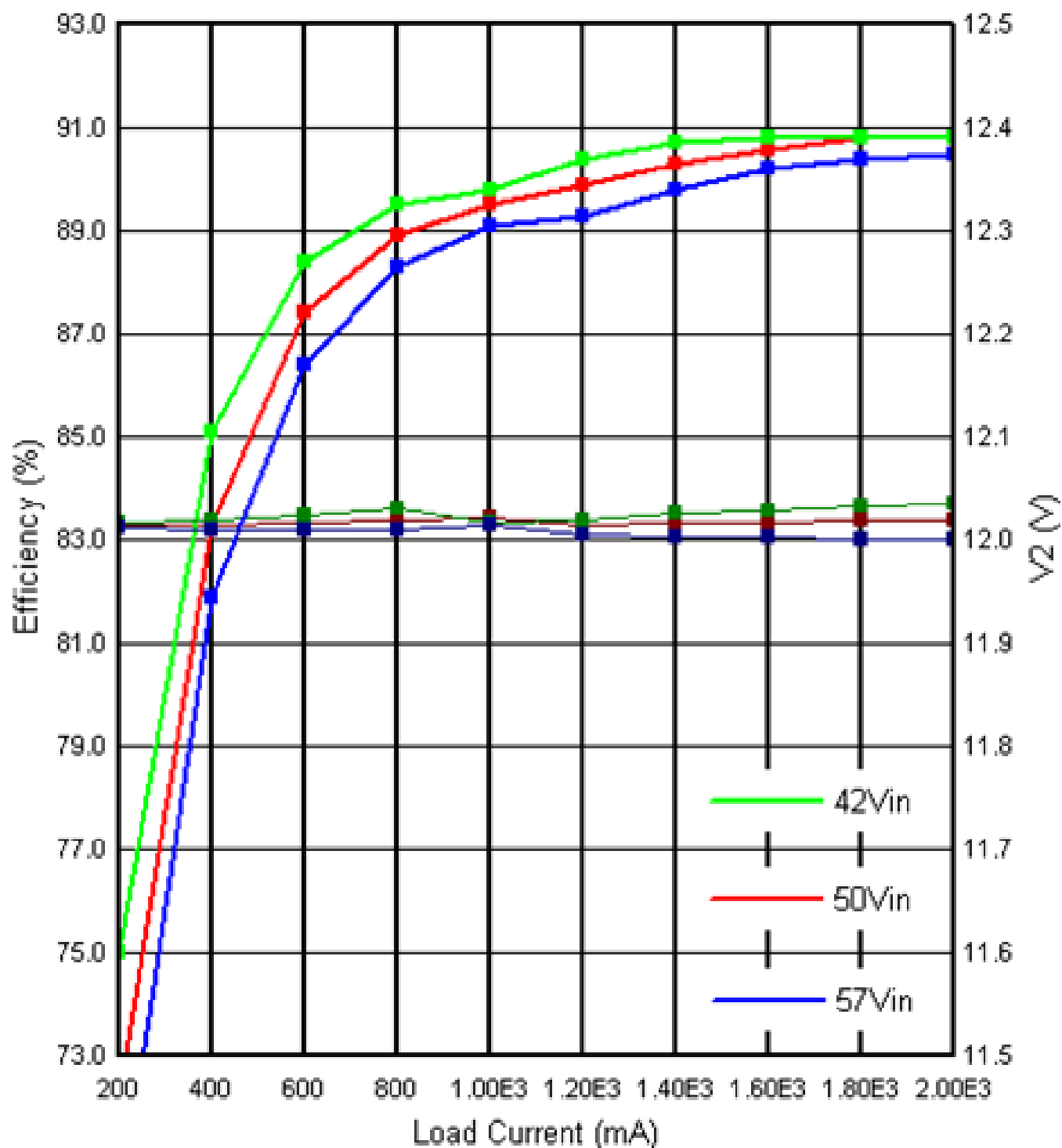
Figure 3. Efficiency (not including Diode Bridge) and Output Voltage (V2) Regulation
