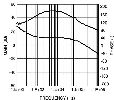
Figure 8-5. Error Amplifier Gain and Phase
