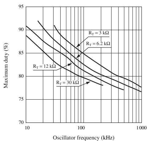
Maximum output duty — Oscillator frequency
