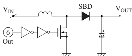
Figure 1. Output bootstrap circuit
