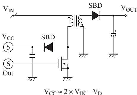
Figure 2. Gate drive voltage bootstrap technique
