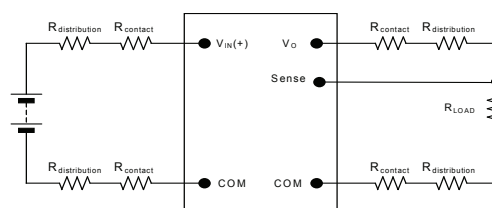
Figure 31. Remote sense circuit configuration
