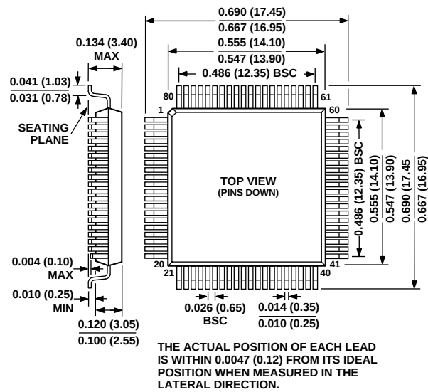
ADSP-216x 80-Lead Plastic Quad Flatpack (MQFP)
