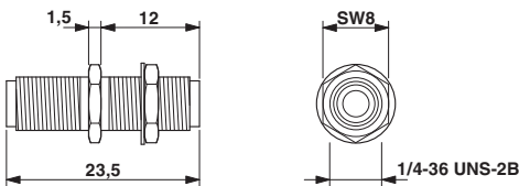
Dimensional drawing F-SMA coupling
