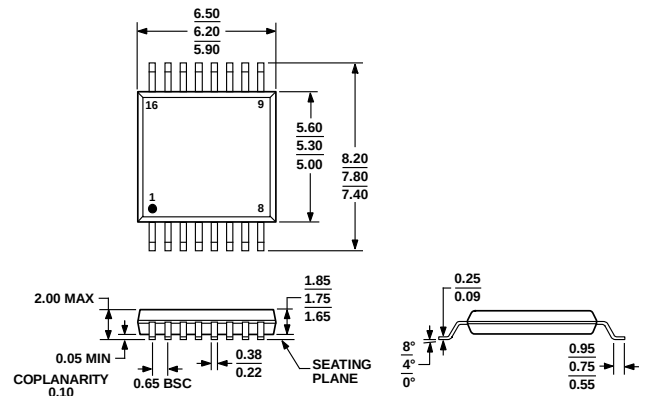
Figure 43. 16-Lead Shrink Small Outline Package [SSOP] (RS-16) Dimensions shown in millimeters
