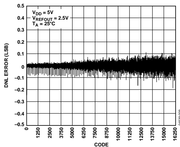
Figure 10. DNL—AD5640-2/AD5640-3
