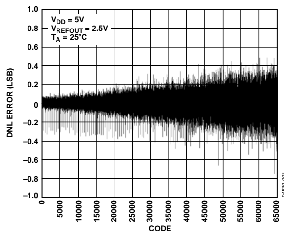
Figure 9. DNL—AD5660-2/AD5660-3
