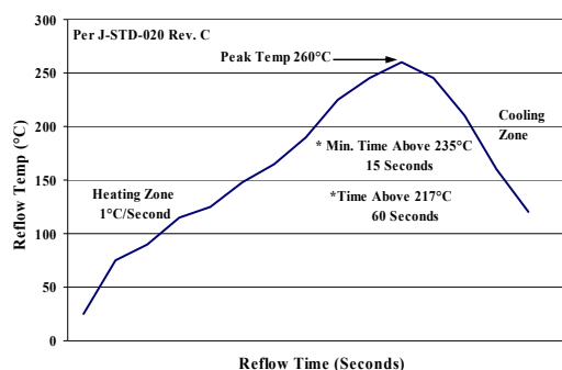
Figure 41. Recommended linear reflow profile using Sn/Ag/Cu solder.
