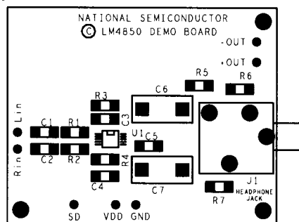
Figure 44. Recommended MM PC Board Layout: Component-Side SilkScreen
