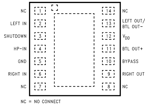
Figure 4. Top View 14 Lead WSON See Package Number NHE0014A
