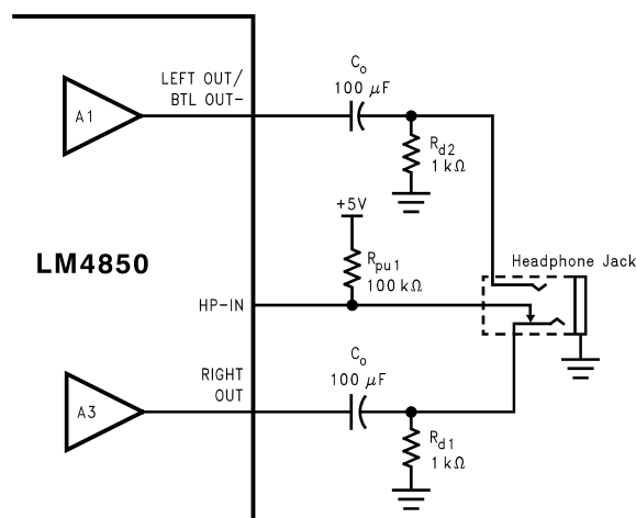
Figure 40. Headphone Control Circuit
