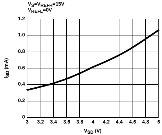
FIGURE 2. DIGITAL SUPPLY VOLTAGE vs DIGITAL SUPPLY CURRENT
