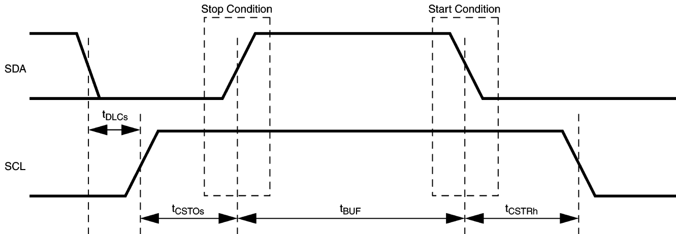
Figure 14. ACCESS.bus Start and Stop Condition Timing
