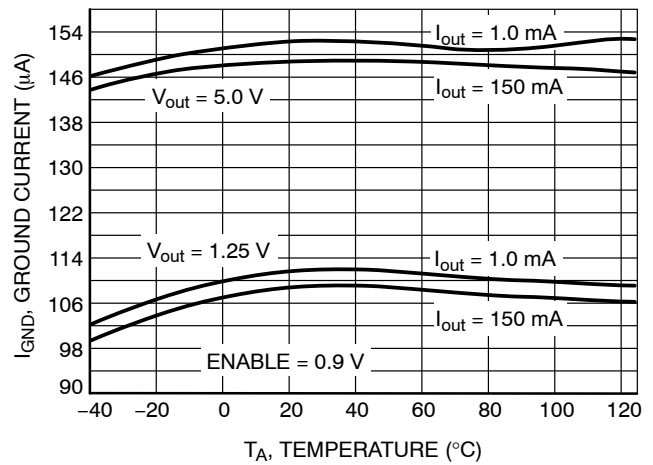
Figure 18. Ground Current (Run Mode) vs. Temperature
