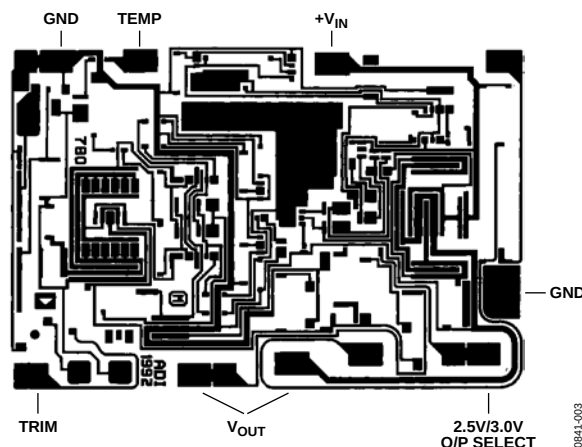
Figure 3. Die Layout
