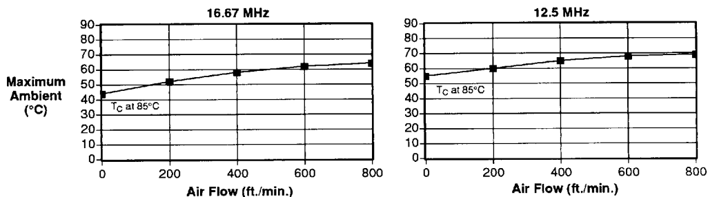
Figure 2. Am29205 Microcontroller—Maximum Allowable Ambient Temperature (Data Sheet Limit, I_{CCOPmax} , V_{CC}=+5.25 V, Average Thermal Impedance)
