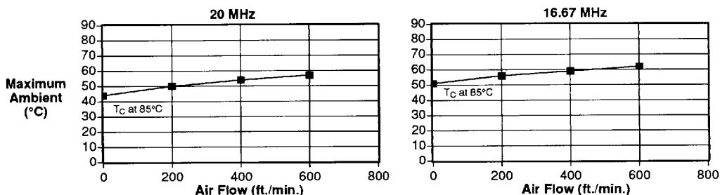
Figure 1. Am29200 Microcontroller—Maximum Allowable Ambient Temperature (Data Sheet Limit, I_{CCOPmax} , V_{CC}=+5.25 V, Average Thermal Impedance)
