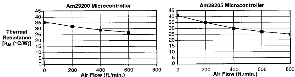
Figure 3. Thermal Impedance
