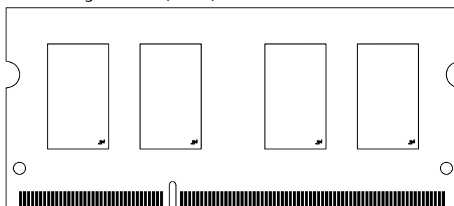
Figure 1: 204-Pin SODIMM (MO-268 R/C A)
