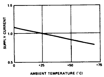
Typical Supply Current vs. Temperature, Normalized [2]
