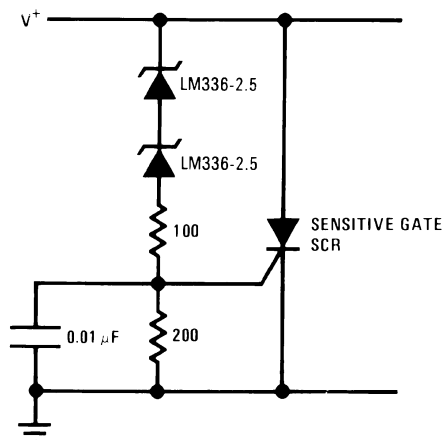
Figure 18. 5V Crowbar
