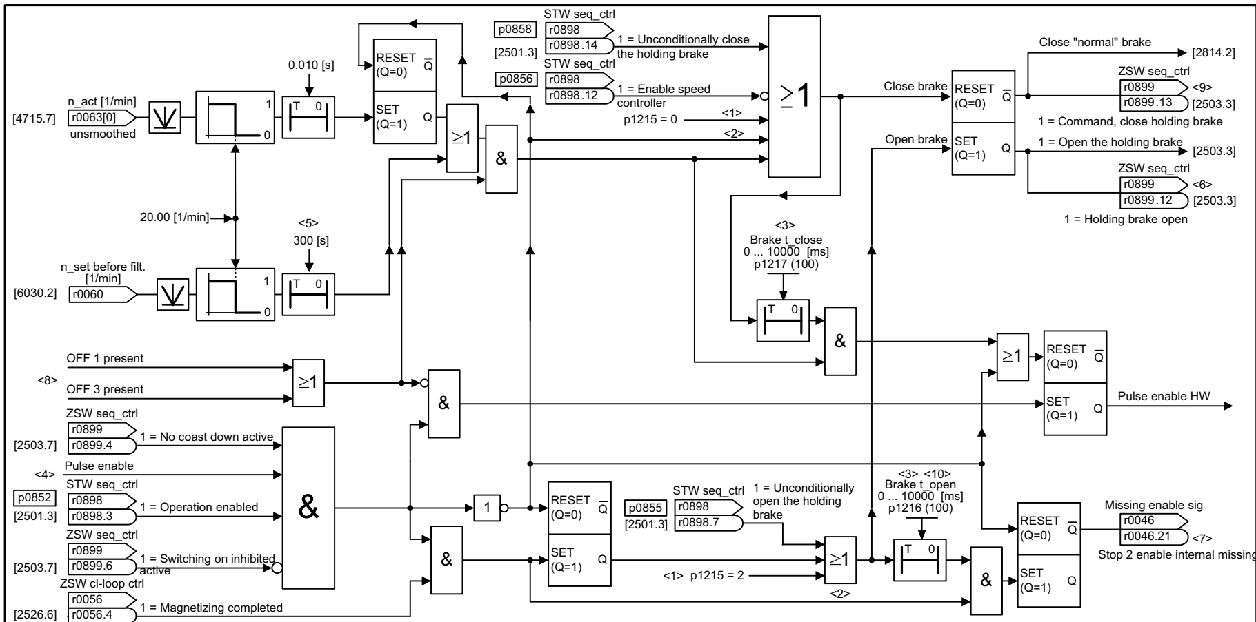
Fig. 2-56 2701 – Basic braking control
