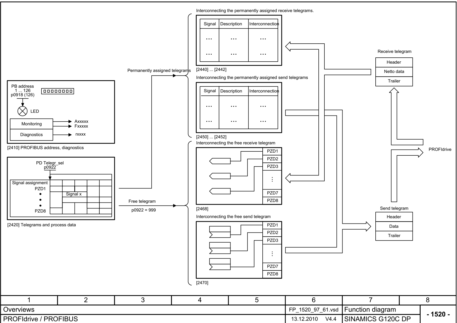
Fig. 2-5 1520 – PROFIdrive/PROFIBUS
