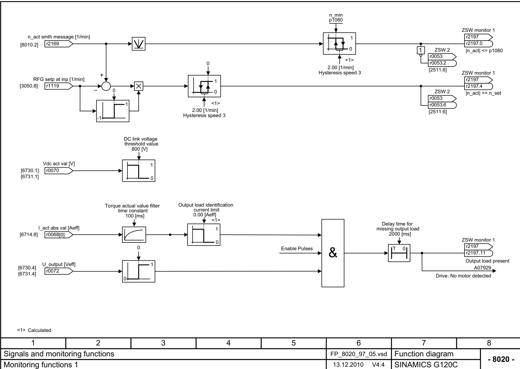
Fig. 2-98 8020 – Monitoring functions 1
