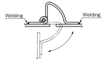
Layout of Installation
