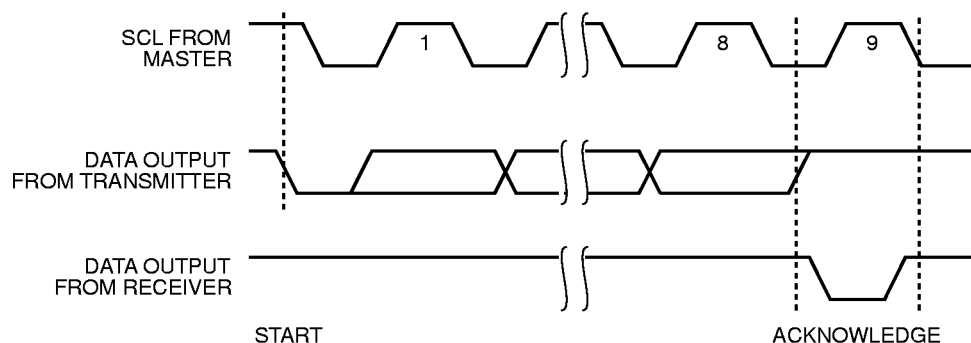
Figure 5. Acknowledge Timing
