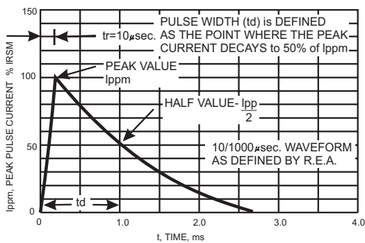
FIG.3- PULSE WAVEFORM
