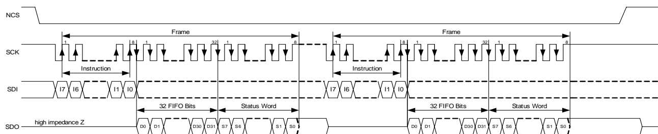
Figure 64 Read FIFO
