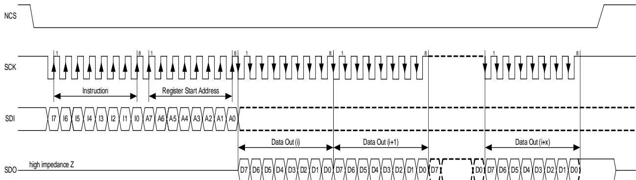
Figure 60 Burst Read Registers
