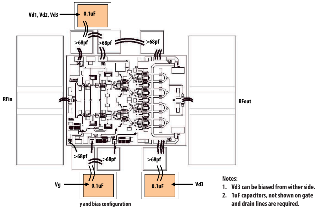
Figure 13. Typical Assembly and bias configuration
