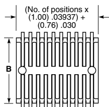
-06 & -10 Contact Detail
