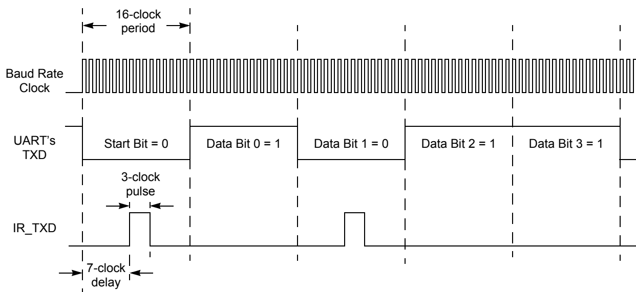
Figure 28. Infrared Data Transmission
