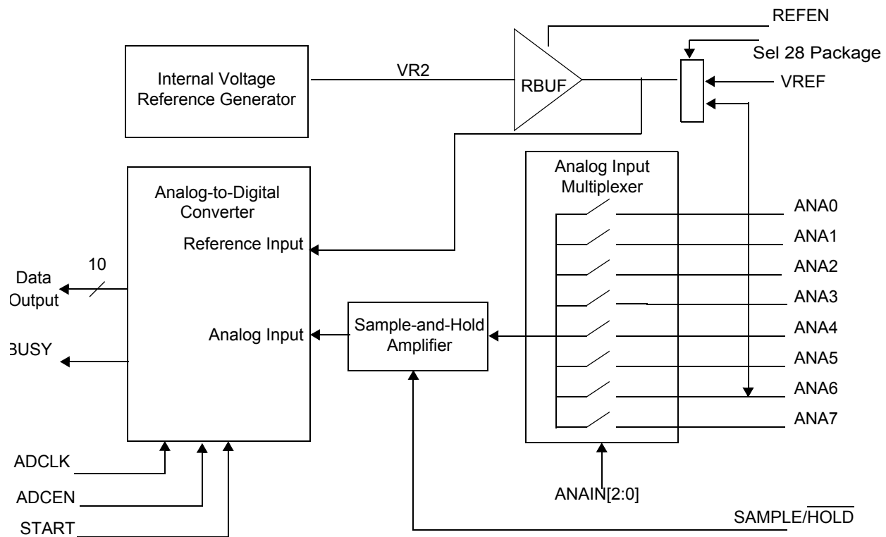
Figure 30. Analog-to-Digital Converter Block Diagram
