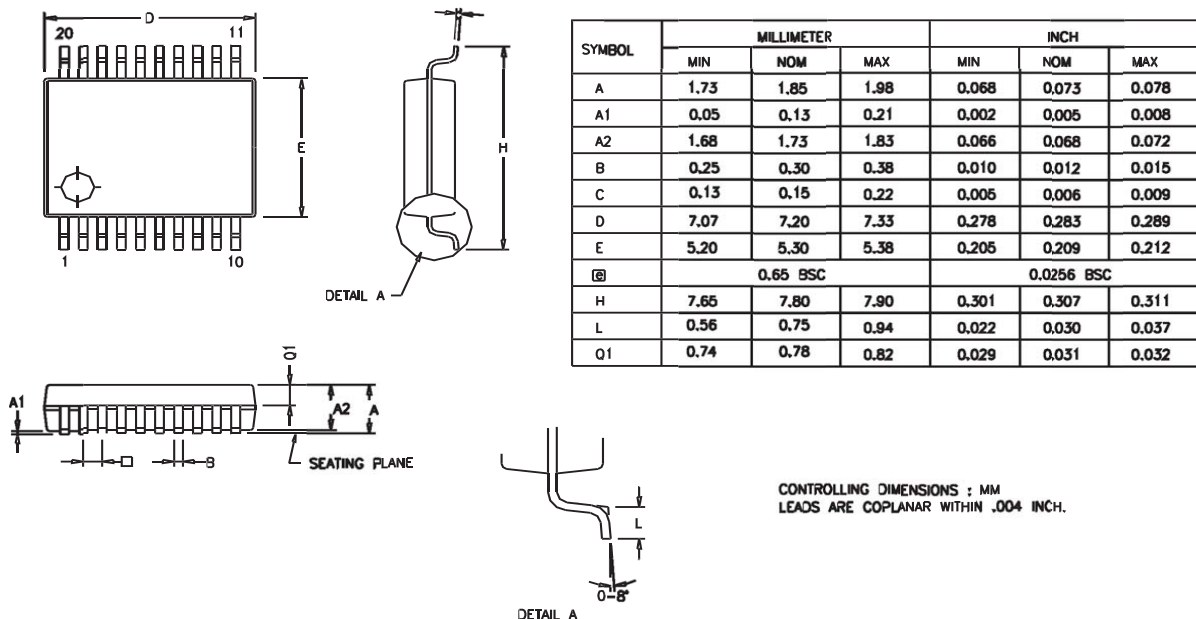
Figure 80. 20-Pin Small Shrink Outline Package (SSOP)
