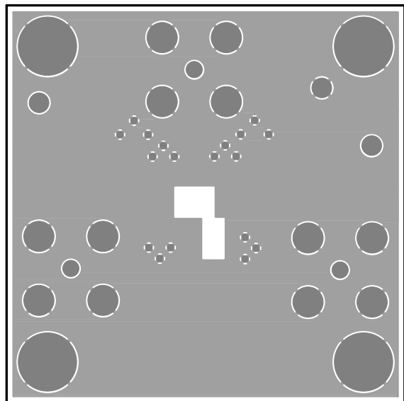
Figure 37. KEB002 (Bottom-side)
