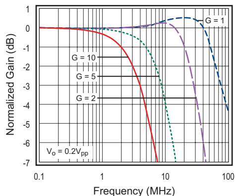
Figure 5. Non-Inverting Freq. Response ( +2.7\text{V} )
