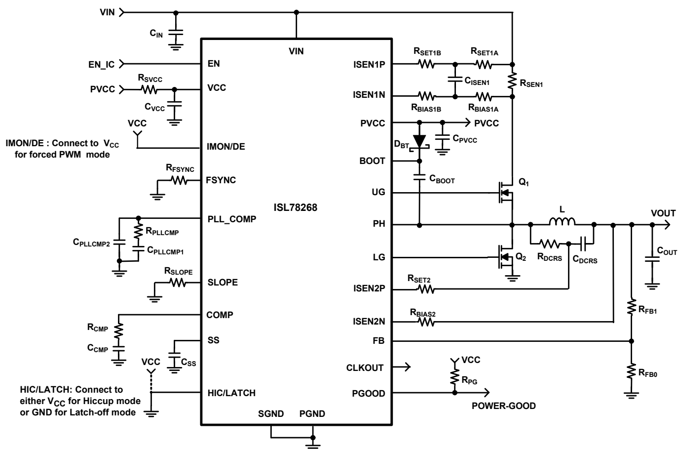
FIGURE 5. SYNCHRONOUS BUCK WITH DCR SENSING
