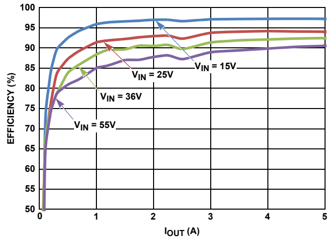
FIGURE 9. EFFICIENCY (AT -40°C): DE MODE, V_{OUT} = 12V , L = 4.7\mu H , f_{SW} = 300kHz
