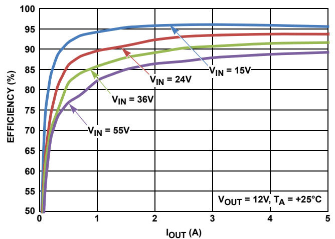
FIGURE 7. EFFICIENCY (AT +25°C): DE MODE, V_{OUT} = 12V , L = 4.7\mu H , f_{SW} = 300kHz
