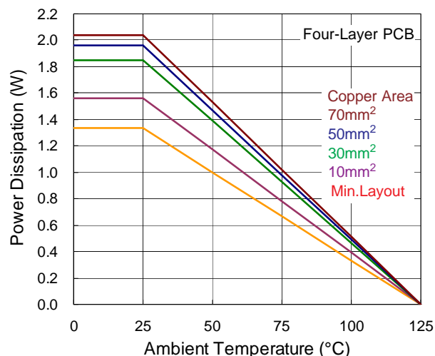
Figure 7. Derating Curves for RT8295B Package
