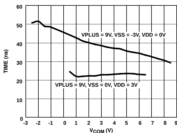
FIGURE 32. t_{ON} vs V_{COM}
