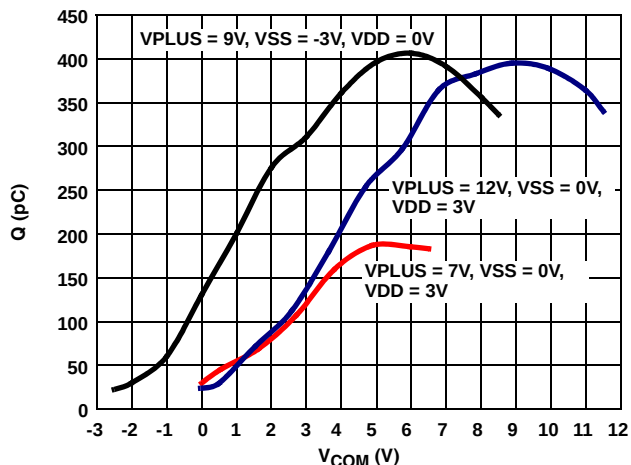
FIGURE 31. CHARGE INJECTION vs SWITCH VOLTAGE
