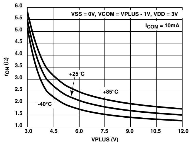
FIGURE 28. ON-RESISTANCE vs SUPPLY VOLTAGE
