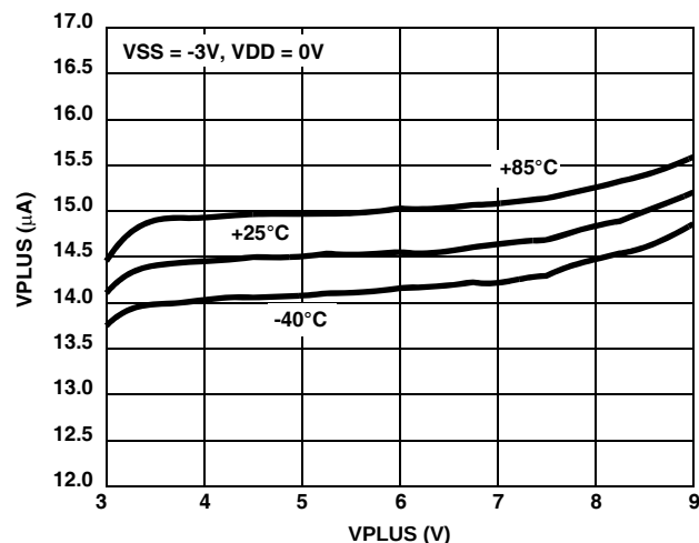
FIGURE 30. DEVICE QUIESCENT CURRENT ( V_{PLUS} )
