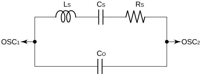
Ceramic Oscillator Parameters
