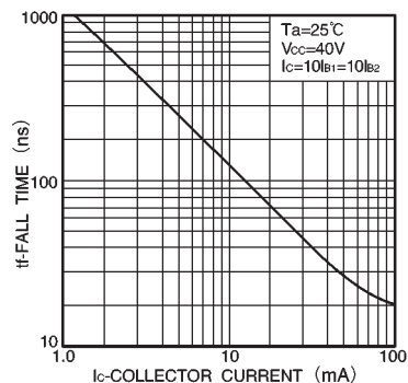
Fig.12 Fall time vs. collector current
