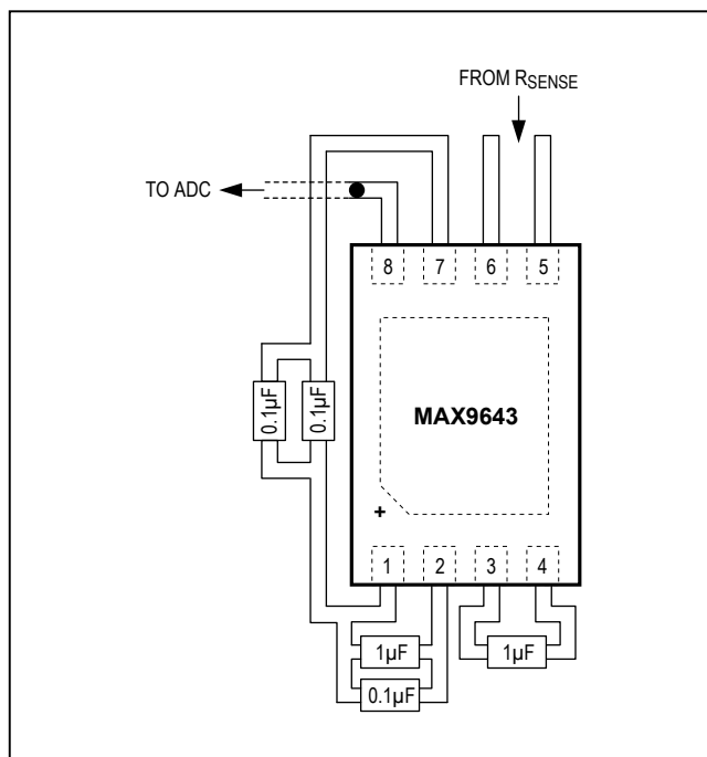
Figure 1. PCB Layout
