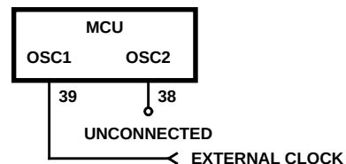
FIGURE 4E. EXTERNAL CLOCK SOURCE CONNECTIONS
