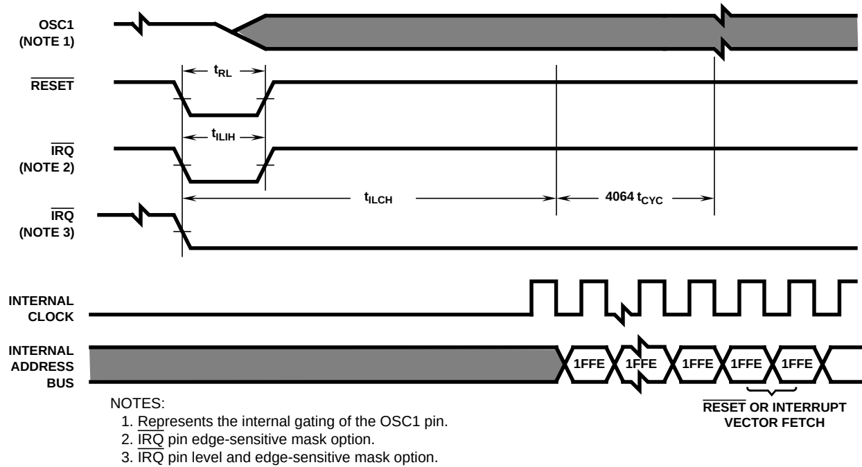
FIGURE 1. STOP RECOVERY TIMING DIAGRAM
