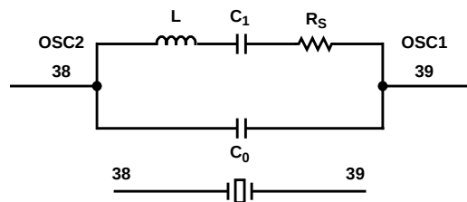
FIGURE 4C. EQUIVALENT CRYSTAL CIRCUIT
