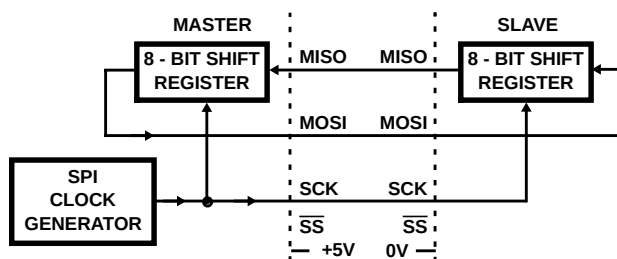
FIGURE 30. SERIAL PERIPHERAL INTERFACE MASTER-SLAVE INTERCONNECTION
