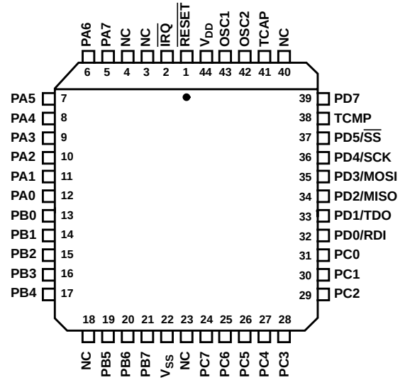
N SUFFIX (PLCC) TOP VIEW
