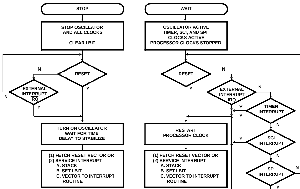
FIGURE 13. STOP/WAIT FLOW DIAGRAM
