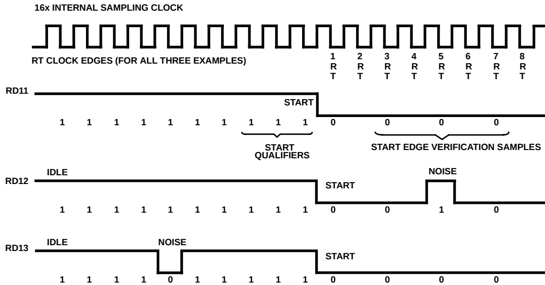
FIGURE 21. EXAMPLES OF START BIT SAMPLING TECHNIQUE
