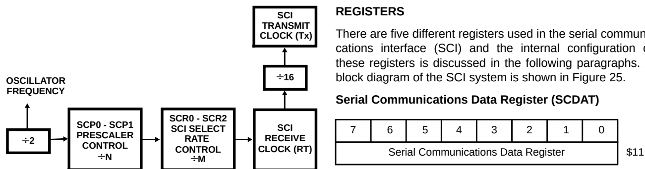
FIGURE 26. RATE GENERATOR DIVISION
