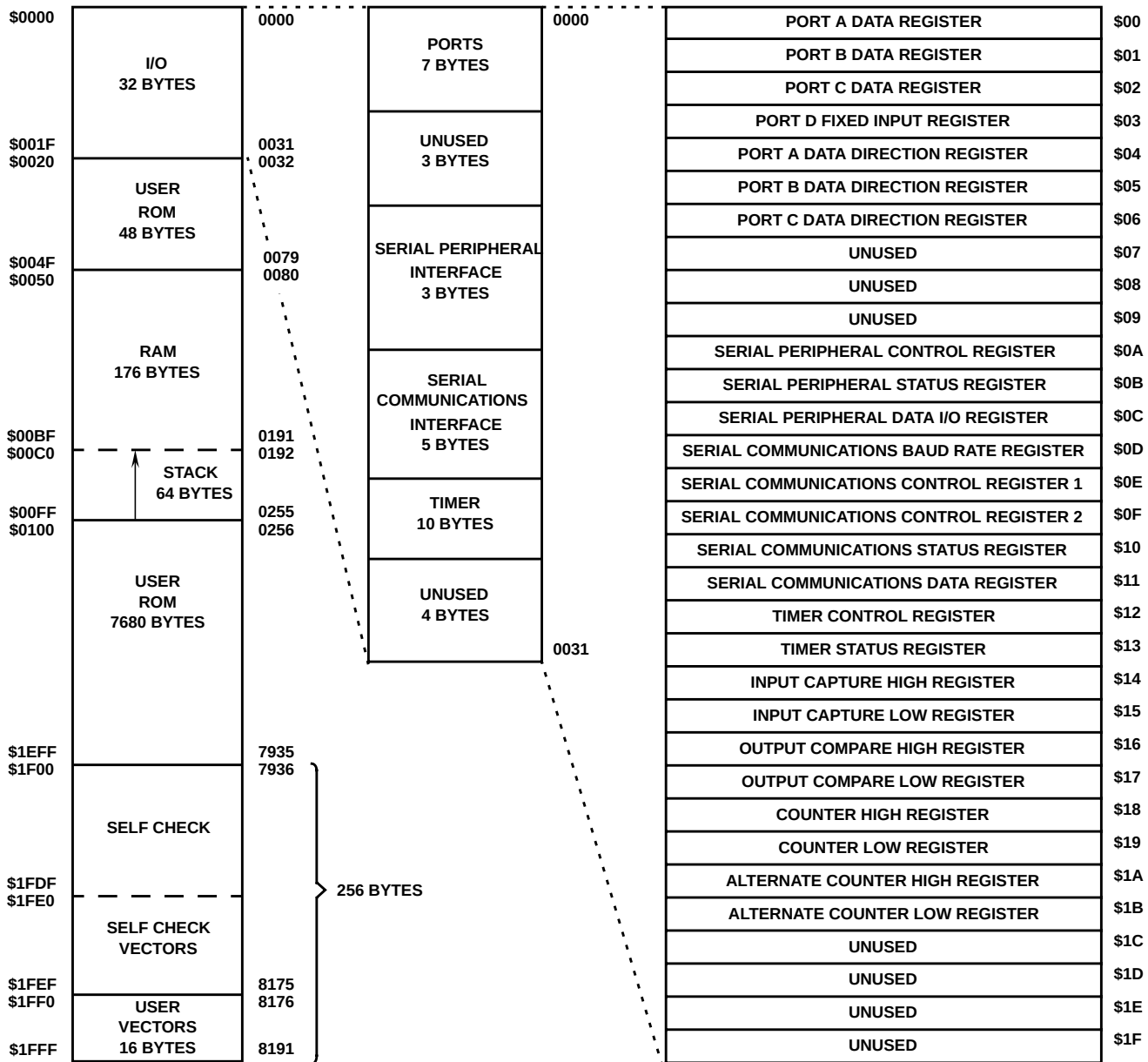
FIGURE 7. ADDRESS MAP FOR CDP68HC05C8, CDP68HCL05C8 AND CDP68HSC05C8
