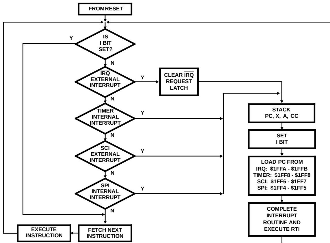
FIGURE 12. HARDWARE INTERRUPT FLOW DIAGRAM
