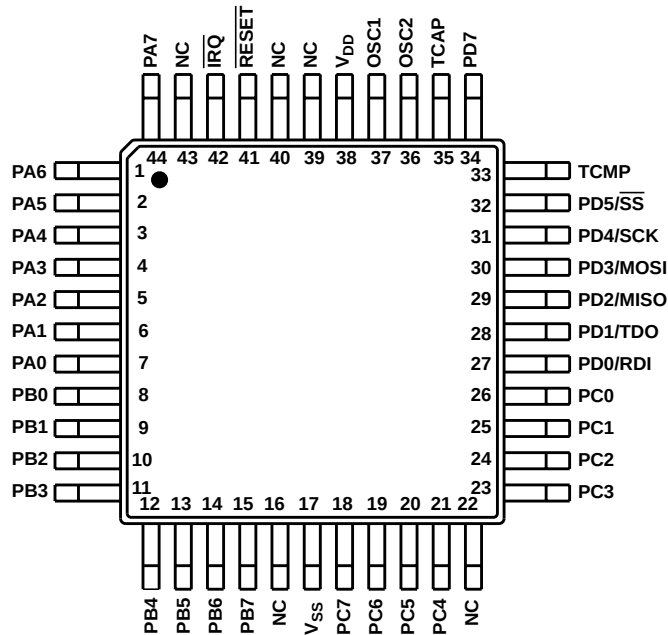
Q SUFFIX (MQFP) TOP VIEW
