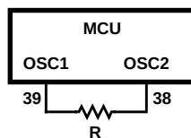
FIGURE 4D. RC OSCILLATOR CONNECTIONS
