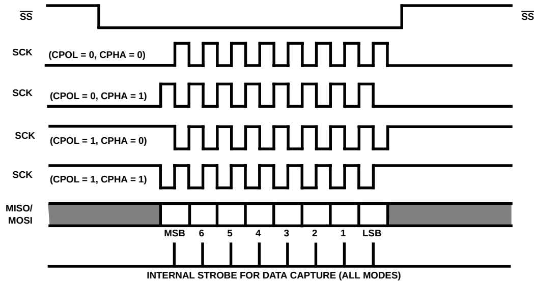
FIGURE 28. DATA CLOCK TIMING DIAGRAM
