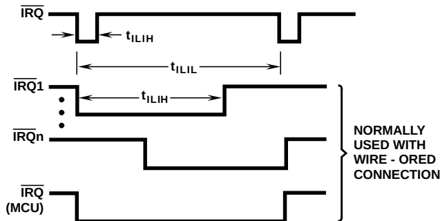
FIGURE 14A. EXTERNAL INTERRUPT FUNCTION DIAGRAM
