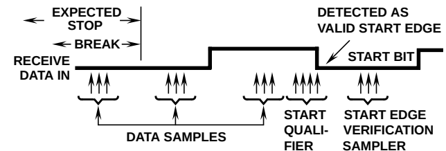
FIGURE 24. SCI START BIT FOLLOWING A BREAK
