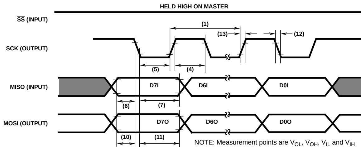
FIGURE 3D. SPI MASTER TIMING CPOL = 1, CPHA = 0
