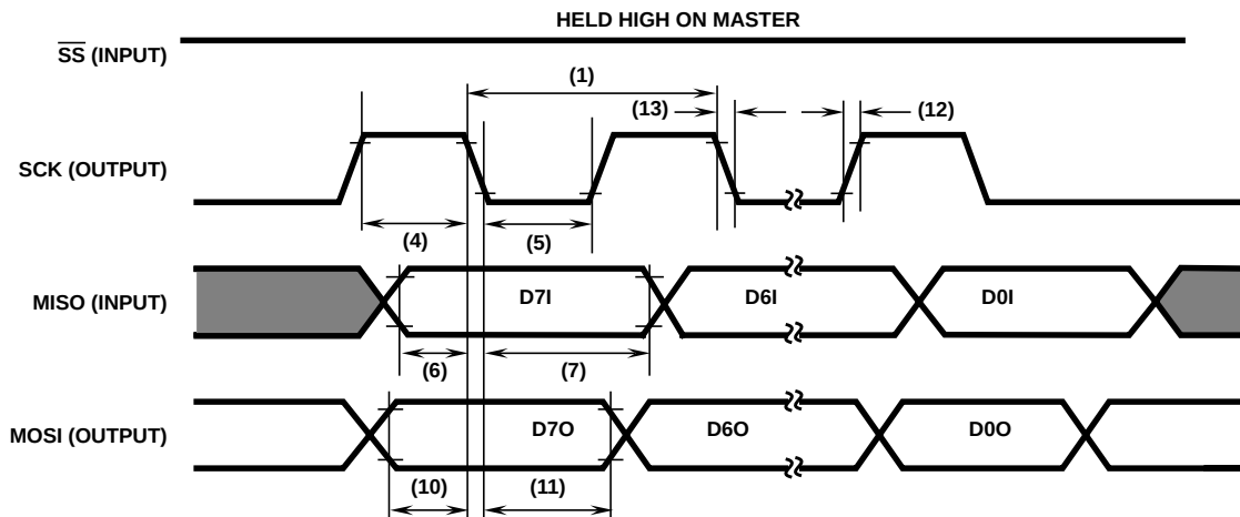
FIGURE 3A. SPI MASTER TIMING CPOL = 0, CPHA = 1
