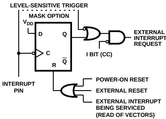
FIGURE 14A. EXTERNAL INTERRUPT FUNCTION DIAGRAM
