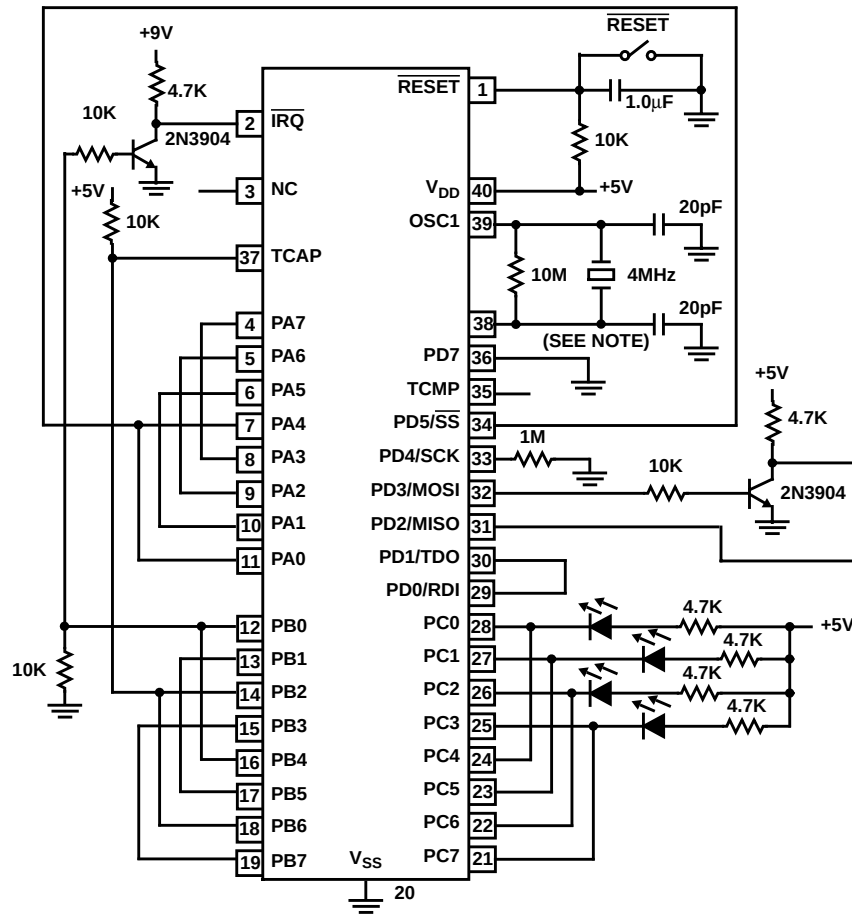
FIGURE 10. SELF-CHECK CIRCUIT SCHEMATIC DIAGRAM
