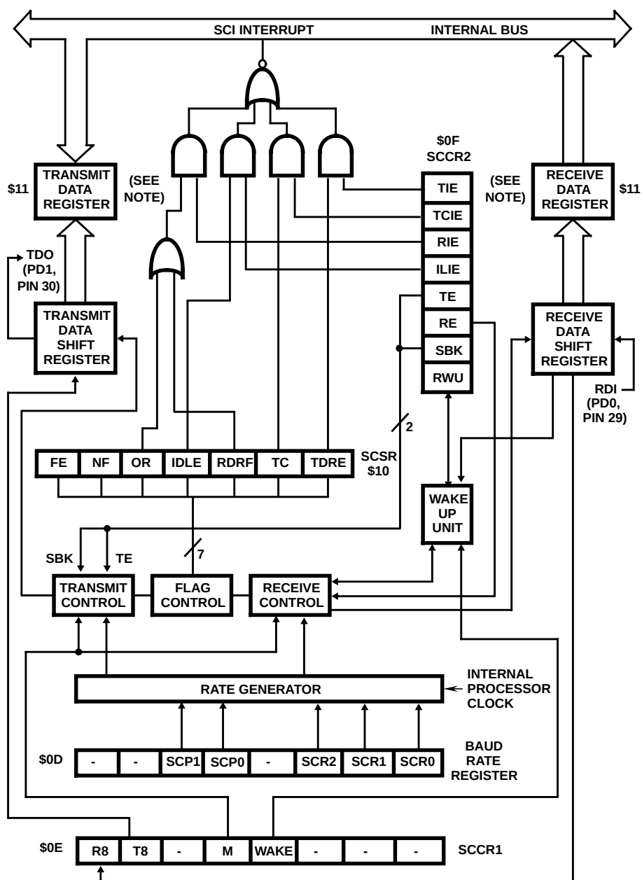
FIGURE 25. SERIAL COMMUNICATIONS INTERFACE BLOCK DIAGRAM
