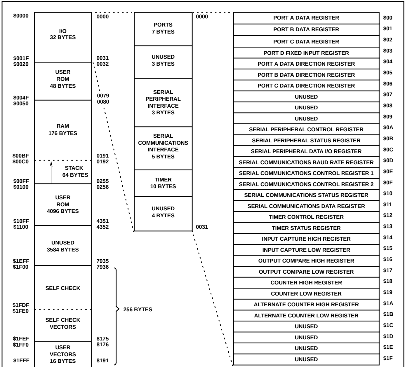
FIGURE 6. ADDRESS MAP FOR CDP68HC05C4, CDP68HCL05C4 AND CDP68HSC05C4
