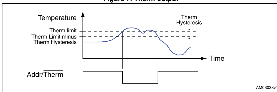
Figure 7. \overline{\text{Therm}} output
