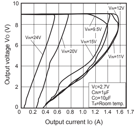
Fig.7 Overcurrent Protection Characteristics (PQ090DNA1ZPH)
