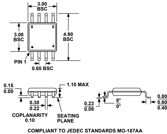
Figure 25. 8-Lead Micro Small Outline Package [MSOP] (RM-8)
