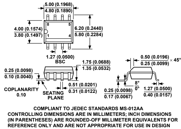
Figure 24. 8-Lead Standard Small Outline Package [SOIC] (R-8)
