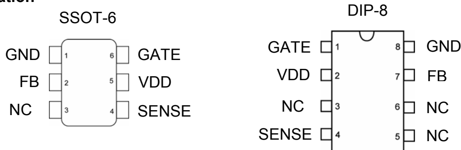
Figure 4. Pin Configurations
