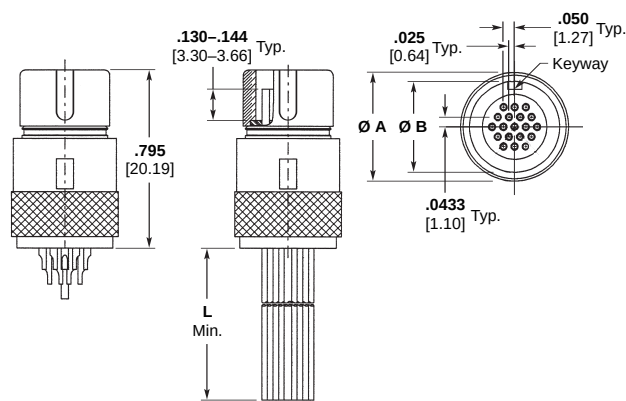
Plug (19 Position Shown)
