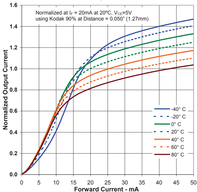
OPB707 - Output Current vs Forward Current vs Temperature
