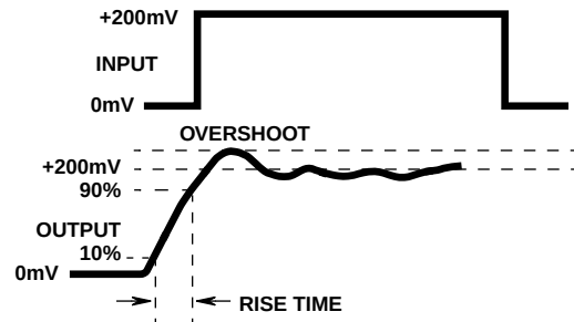
NOTE: Measured on both positive and negative transitions from 0V to +200mV and 0V to -200mV at the output. FIGURE 1. SLEW RATE AND SETTLE TIME
